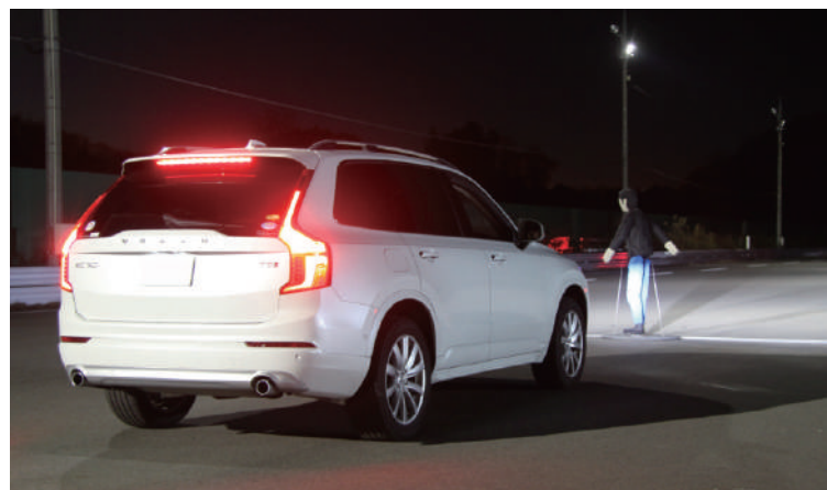
衝突被害軽減ブレーキ(対歩行者[夜間])試験 Evaluation test of autonomous emergency braking (pedestrian [night])
